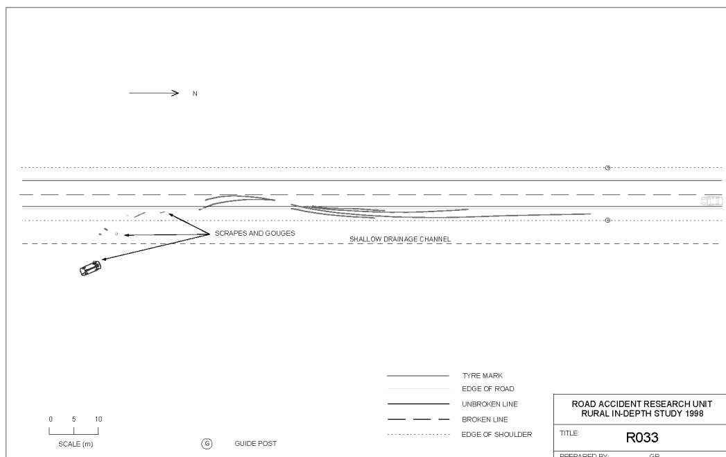
Figure 1 Site diagram showing tyre marks from initial off road excursion and overcorrection back to the left. Case R033
