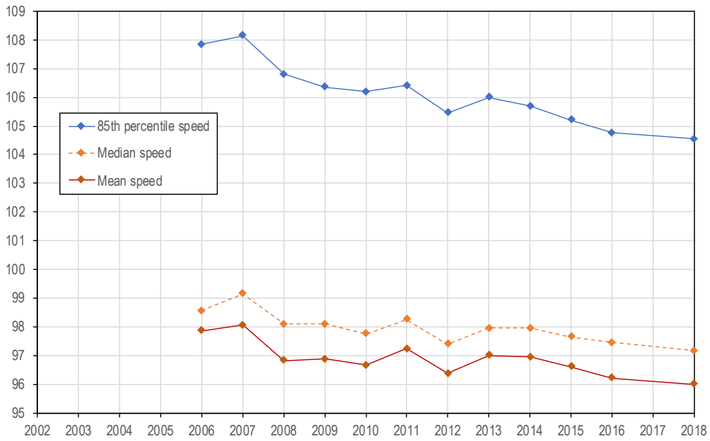
Figure 5.11 Summary speed measurements by year of survey
