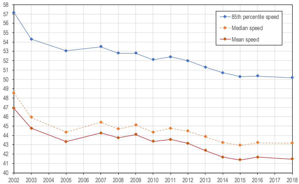
Figure 5.1 Summary speed measurements by year of survey
