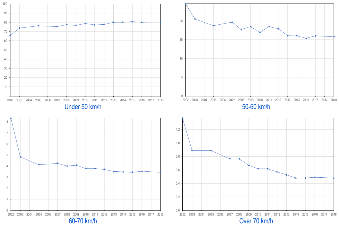
Figure 5.2 Percentage of all vehicles travelling within the given speed ranges by year of survey
