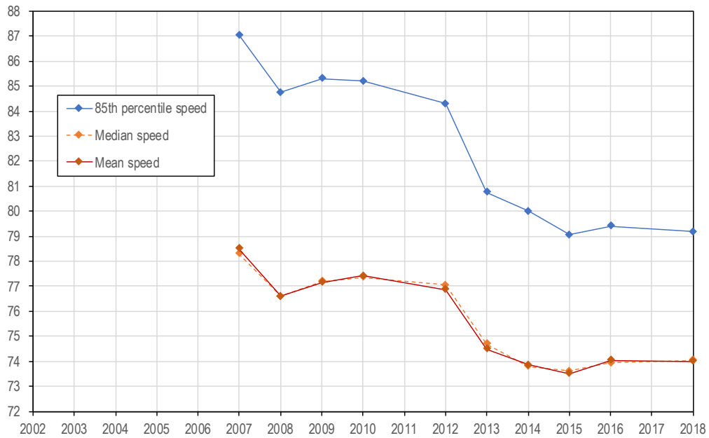
Figure 5.9 Summary speed measurements by year of survey
