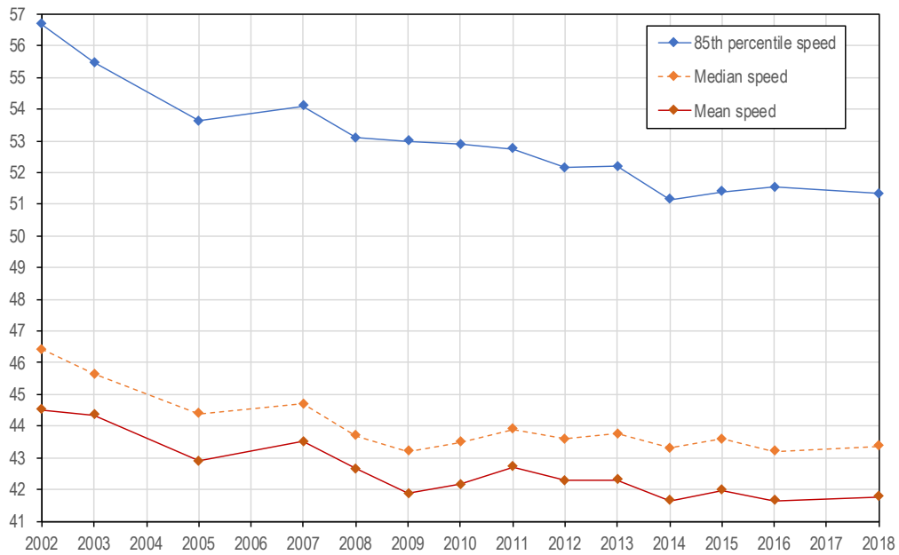
Figure 5.7 Summary speed measurements by year of survey
