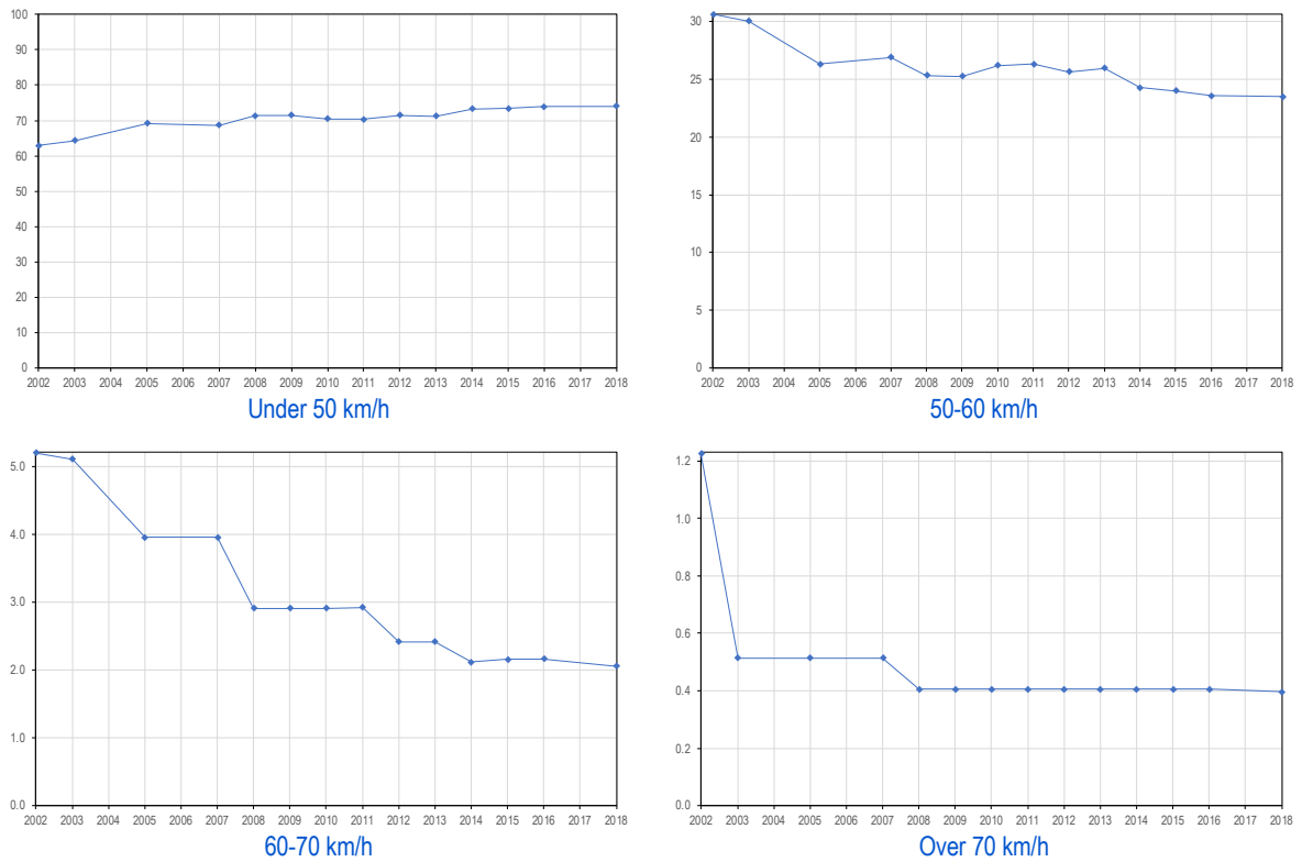
Figure 5.8 Percentage of all vehicles travelling within the given speed ranges by year of survey
