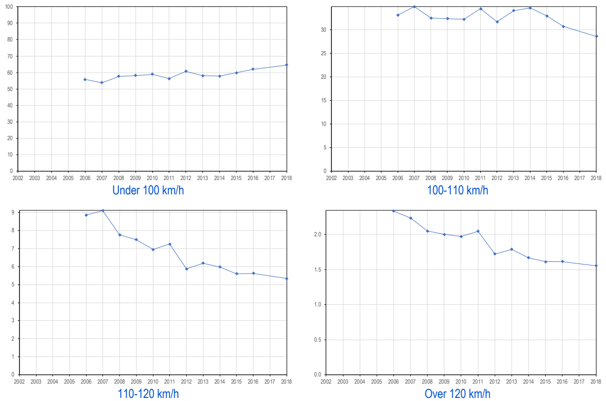
Figure 5.12 Percentage of all vehicles travelling within the given speed ranges by year of survey
