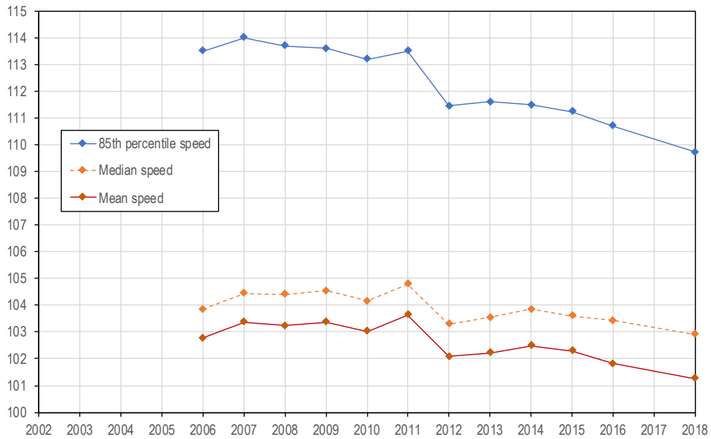
Figure 5.13 Summary speed measurements by year of survey
