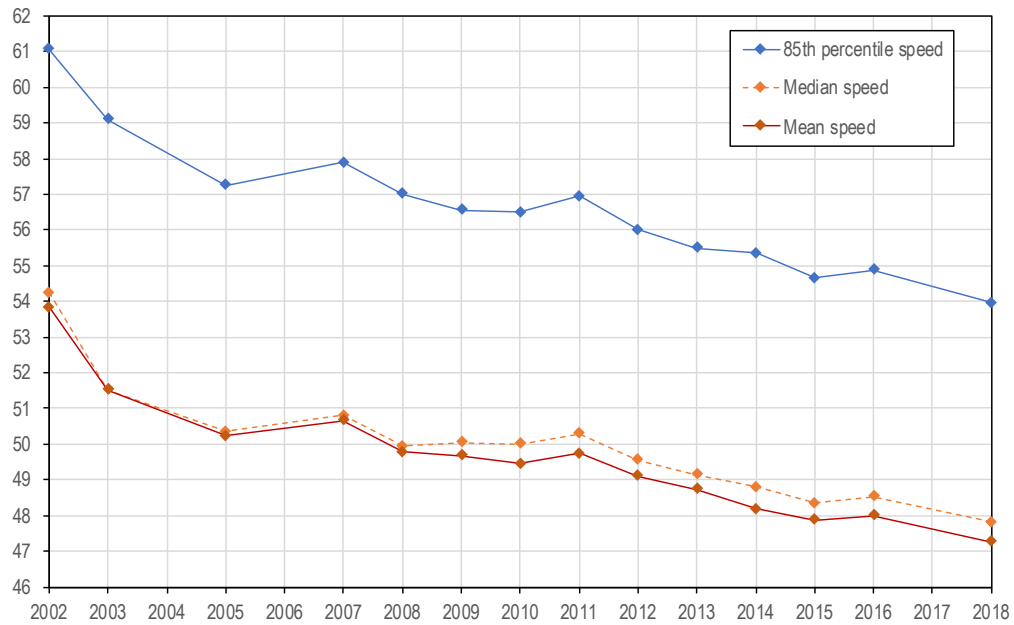
Figure 5.3 Summary speed measurements by year of survey
