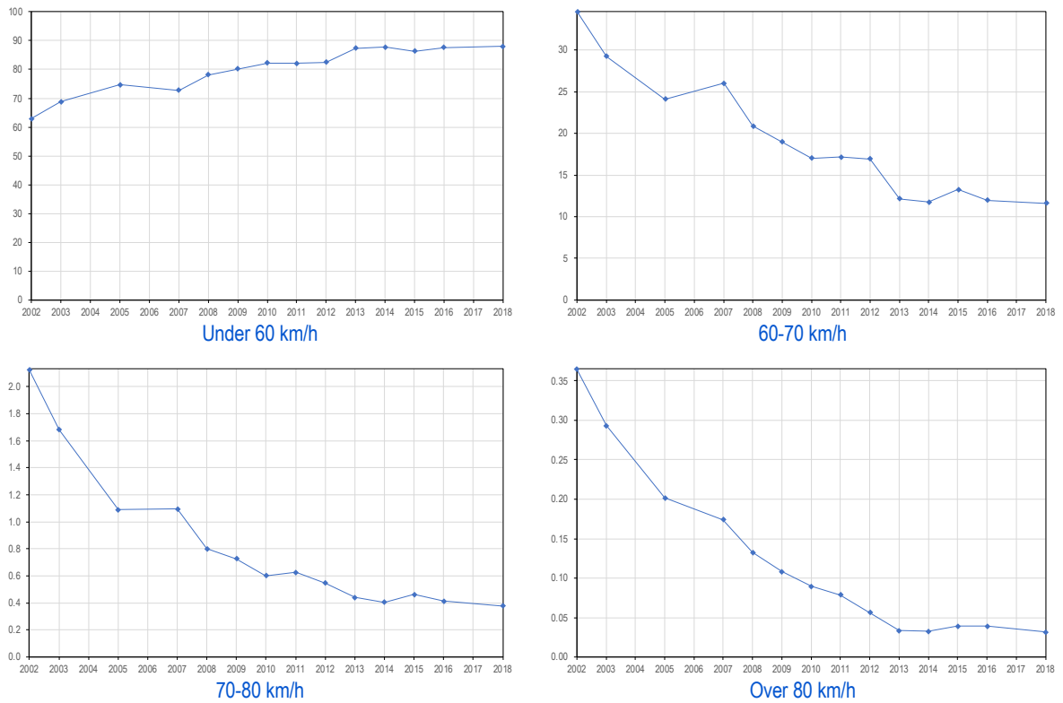
Figure 5.6 Percentage of all vehicles travelling within the given speed ranges by year of survey
