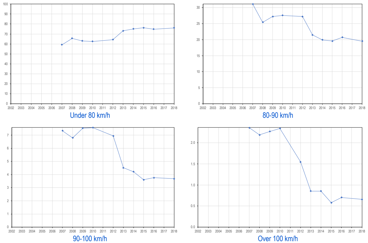
Figure 5.10 Percentage of all vehicles travelling within the given speed ranges by year of survey
