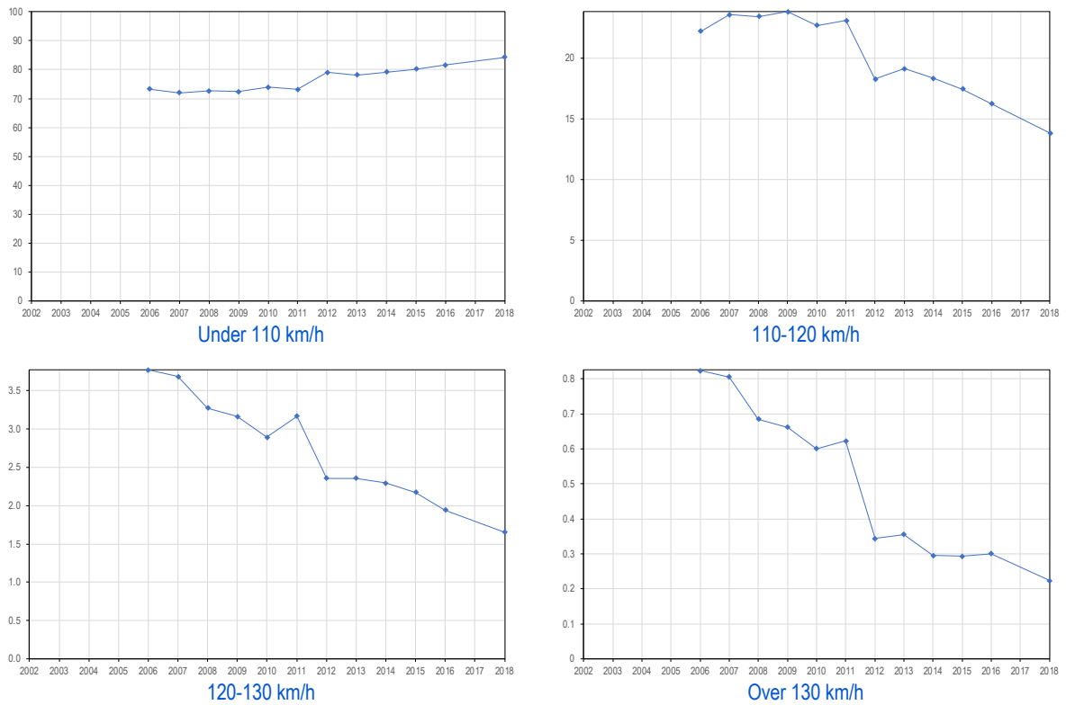
Figure 5.14 Percentage of all vehicles travelling within the given speed ranges by year of survey
