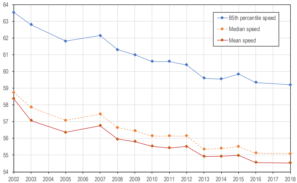
Figure 5.5 Summary speed measurements by year of survey
