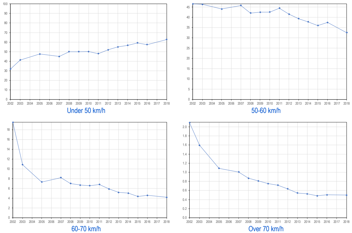
Figure 5.4 Percentage of all vehicles travelling within the given speed ranges by year of survey
